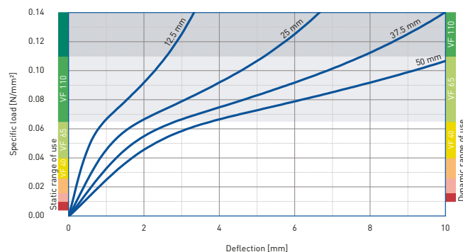
Fig. 2: Quasi-static load deflection curve of a VIKAFoAM material (VF 65)
