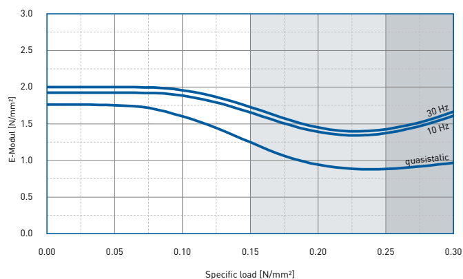
Fig. 7: Modulus of elasticity of a VIKADYN material (VD 150)
